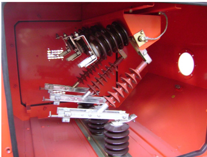
Picture 6 Internal view : option with line disconnecter, equipped with handle device
